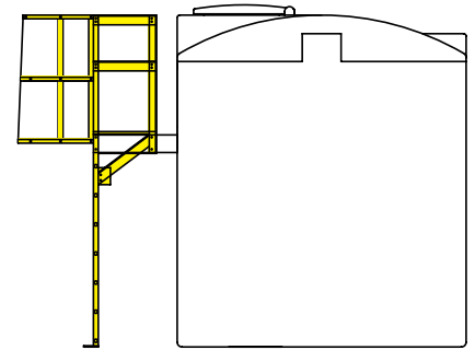
FRP Ladder with Cage & Platform
